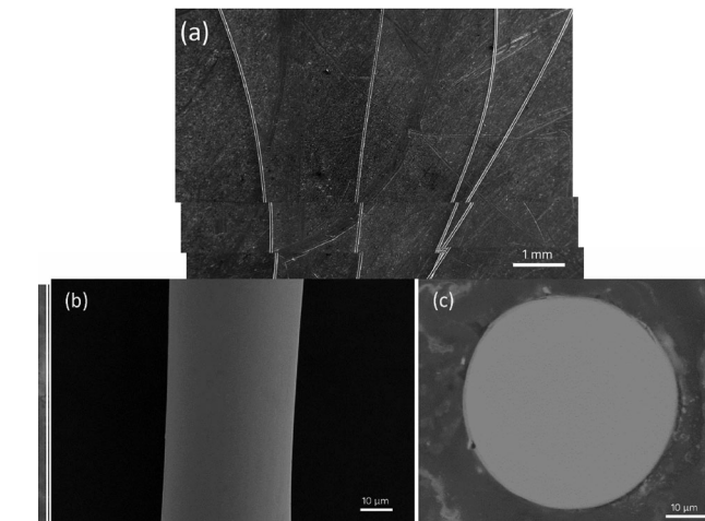
Fig. 1 (a) Optical micrograph of a magnetic glassy film showing a network of dark, elongated magnetic domain walls. A scale bar of 1 mm is shown. (b) SEM image of the surface morphology of the MGF, showing a smooth surface. A scale bar of 10 \mu\text{m} is shown. (c) SEM image of a circular MGF, showing a smooth surface. A scale bar of 10 \mu\text{m} is shown.
